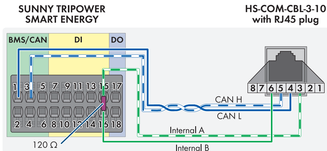
Figure 1: Sunny Tripower Smart Energy with SMA Home Storage when using the SMA HS-COM-CBL-3-10 cable.
