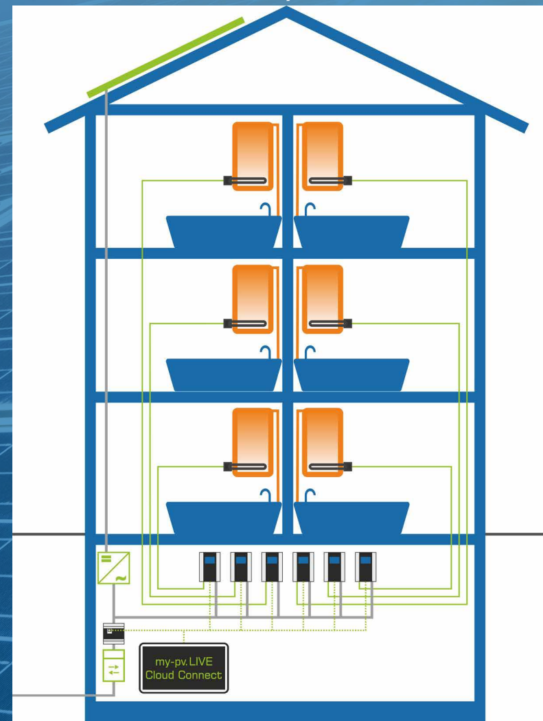
Hot water in on-grid PV-systems with AC•THOR/AC•THOR 9s
