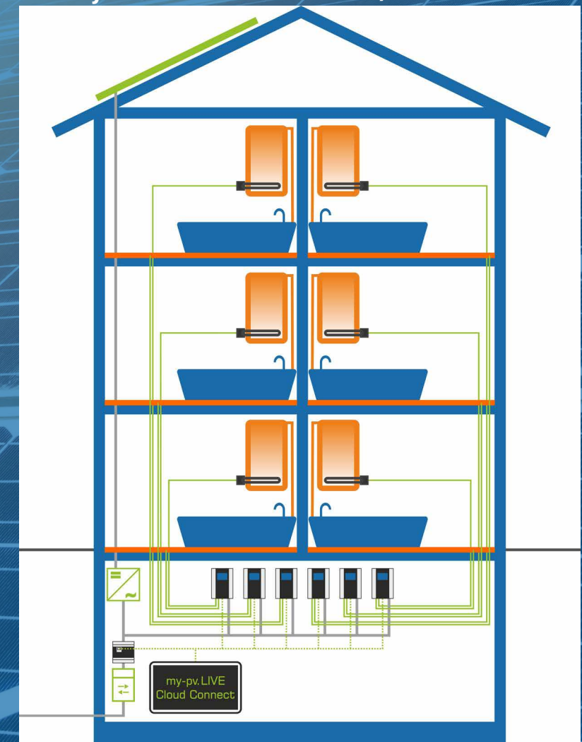
Hot water and heating in on-grid PV-systems with AC•THOR/AC•THOR 9s
